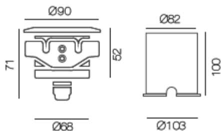
INGROUND UPLIGHT | MINI INGROUND UPLIGHT BLACK
