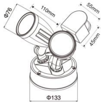
EXTERIOR SPOT LIGHTS | SENTRY TWIN SPOT LIGHT WITH SENSOR 4000K
