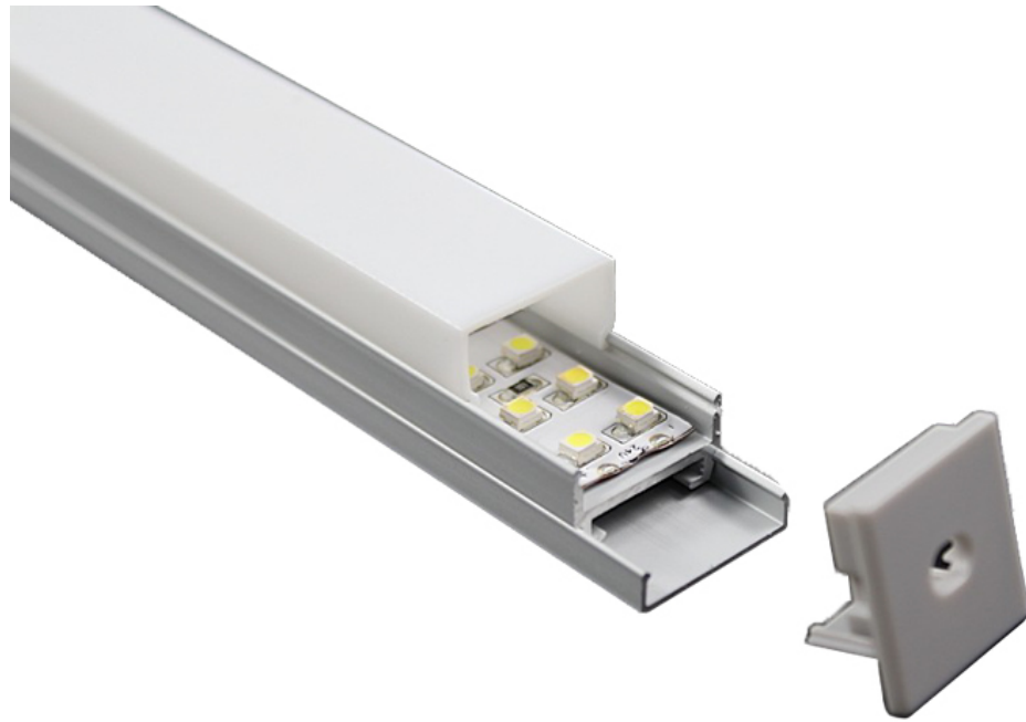
ALUMINIUM EXTRUSION
